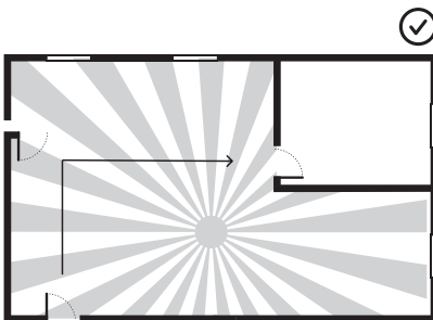
Figure 2: For faster detection, place the sensor away from the pathways between the doors.
