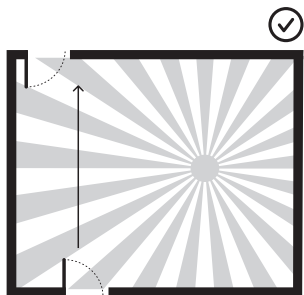
Figure 1: Choose the sensor placement so that people walking from one door to another cross multiple zones.
